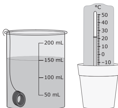
Figure 1. Investigation Setup
