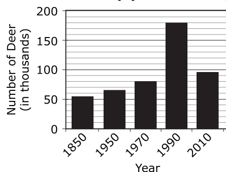
B. White-tailed Deer Population in New Jersey (in thousands)
