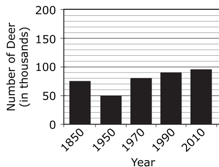
D. White-tailed Deer Population in New Jersey (in thousands)
