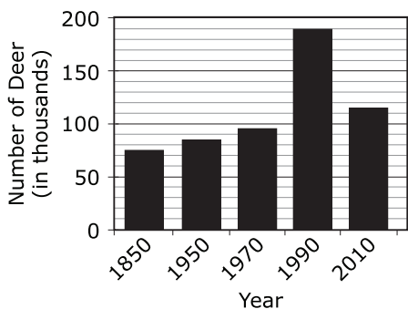
C. White-tailed Deer Population in New Jersey (in thousands)
