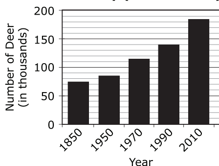
A. White-tailed Deer Population in New Jersey (in thousands)
